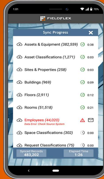
Bulletproof Data Synchronization
